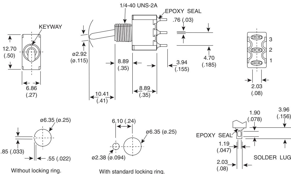
PANEL MOUNTING
